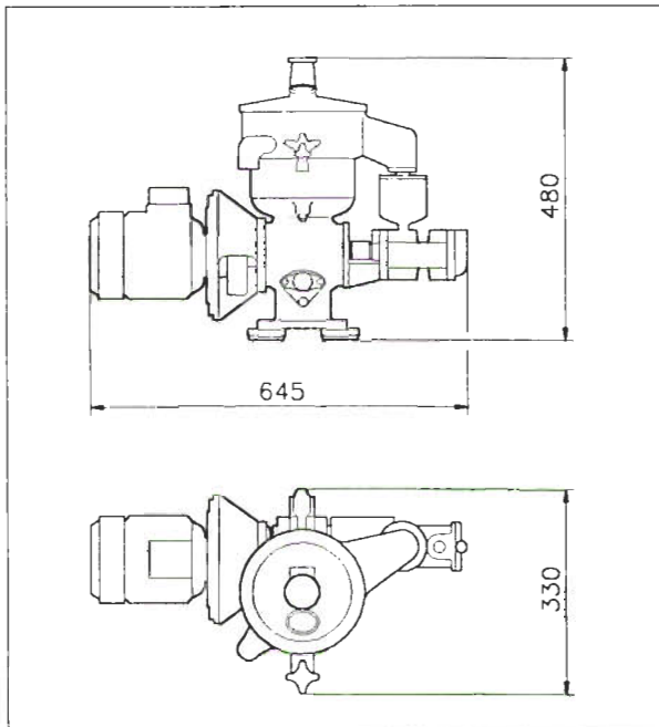
Fig.3 Dimension drawing
